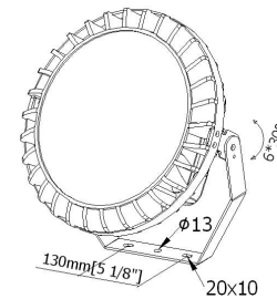
Shown with optional yoke
